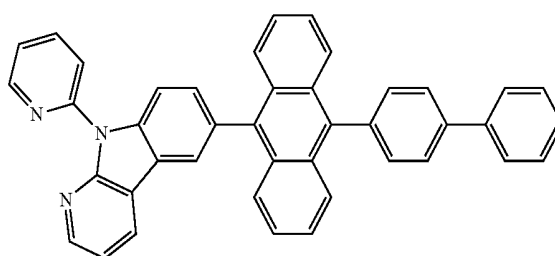
NCGL_A
