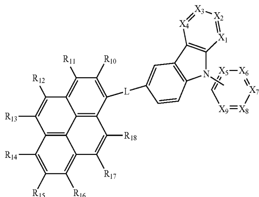
[Chemical Formula 15]
