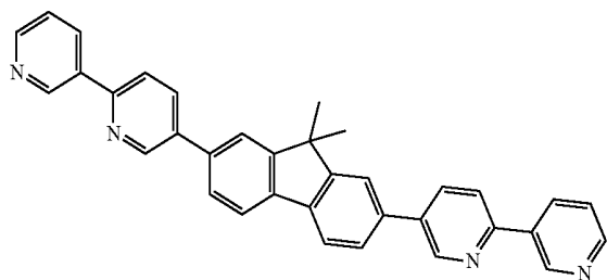
NCGL_C
