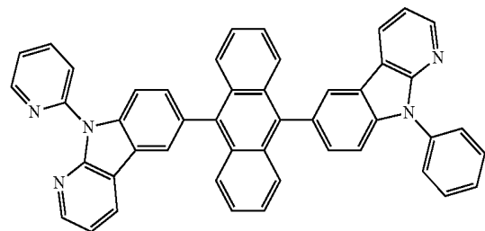
NCGL_C
