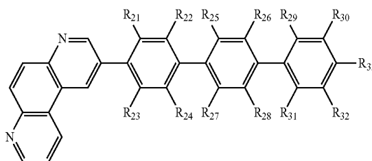
[Chemical Formula 18]
