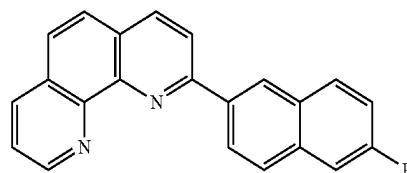
[Chemical Formula 5]
