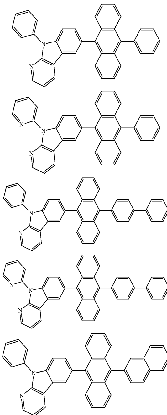
[Chemical Formula 24]
