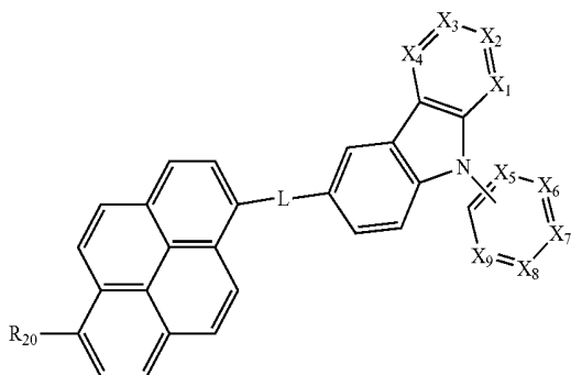
[Chemical Formula 25]
