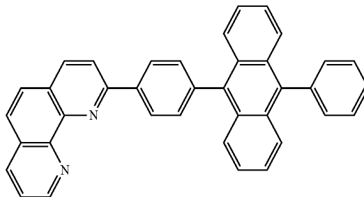
NCGL_A
