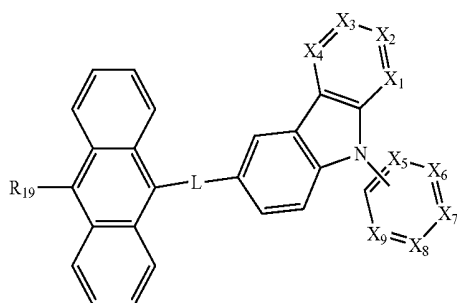
[Chemical Formula 25]
