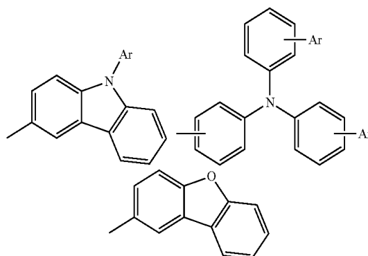
[Chemical Formula 2]
