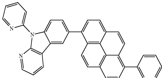
NCGL_B
