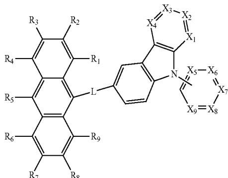
[Chemical Formula 14]
