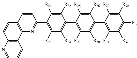
[Chemical Formula 19]
