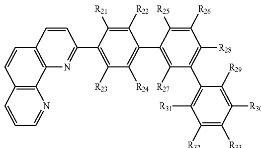
[Chemical Formula 20]
