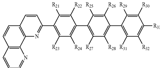
[Chemical Formula 17]
