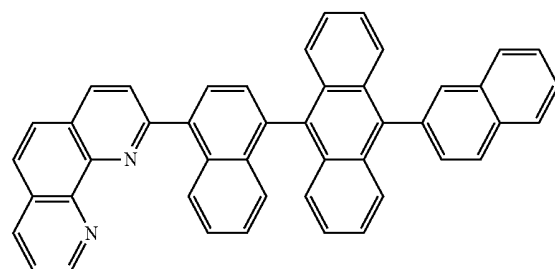
NCGL_C
