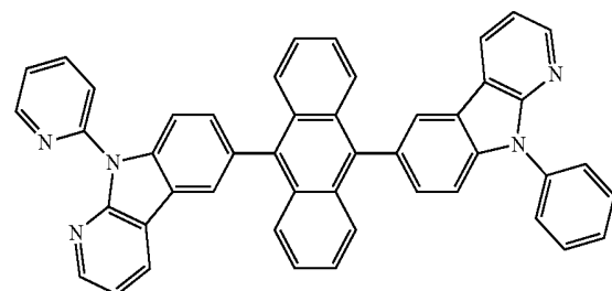
NCGL_C
